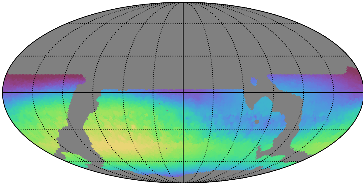
weather_cloudso12v3.4_10yrs WFD u band: Max skyBrightness
