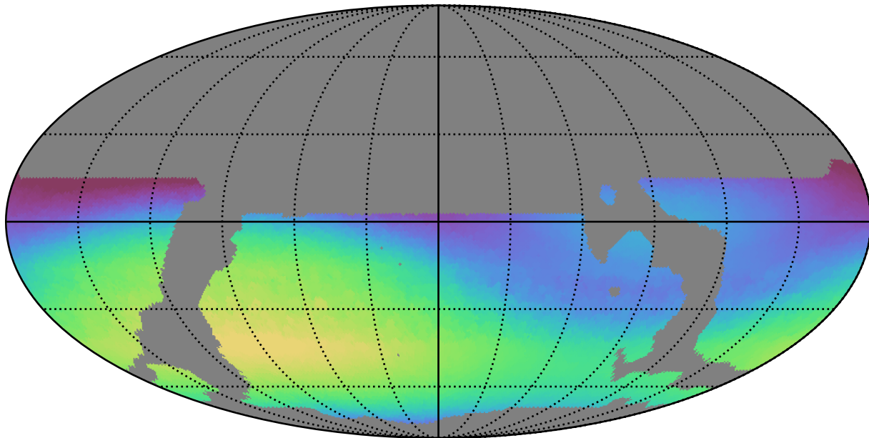
weather_cloudso12v3.4_10yrs WFD r band: Max skyBrightness
