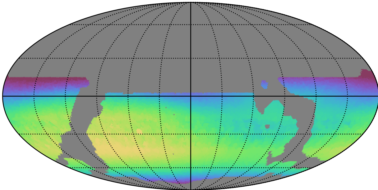
weather_cloudso12v3.4_10yrs WFD i band: Max skyBrightness
