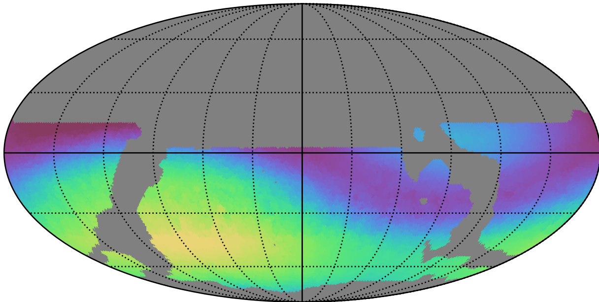
weather_cloudso12v3.4_10yrs WFD g band: Max skyBrightness
