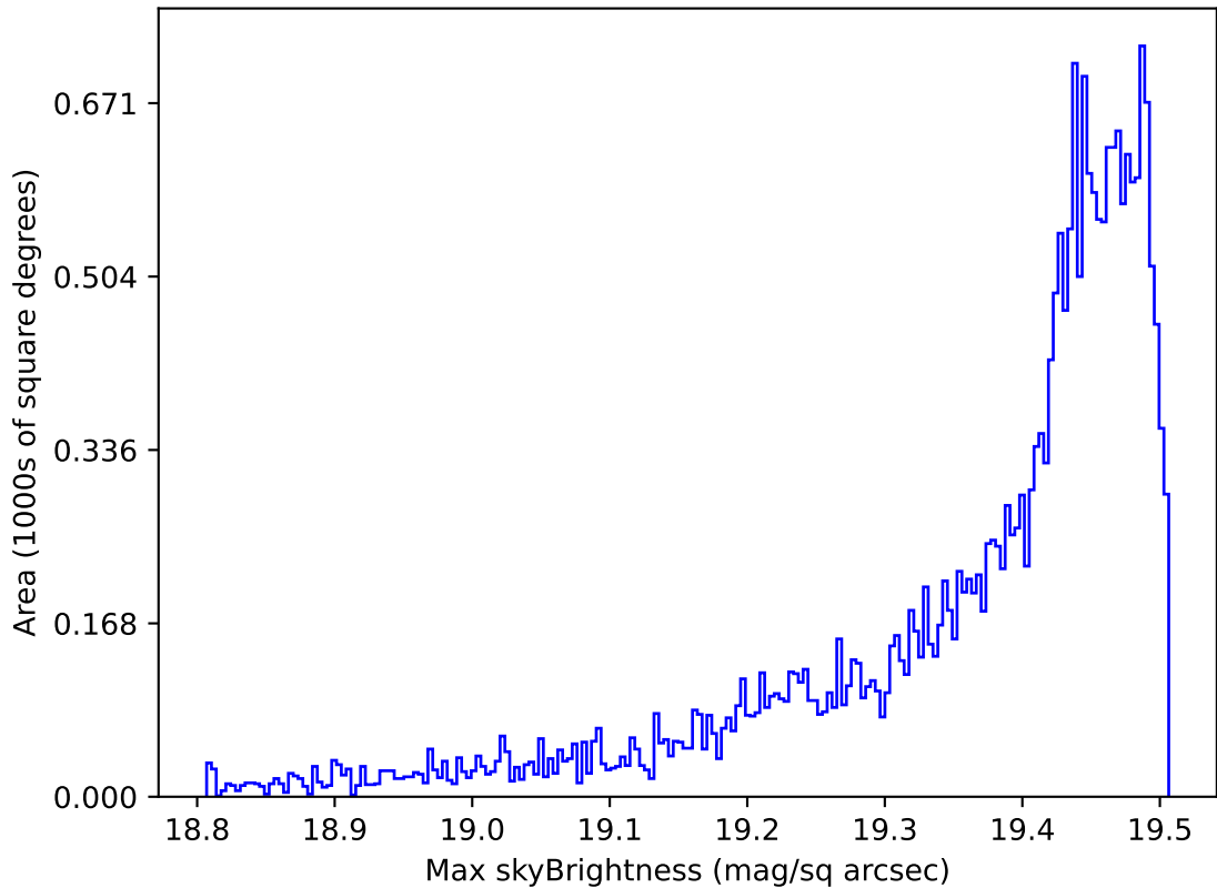
weather_cloudso12v3.4_10yrs All sky z band: Max skyBrightness
