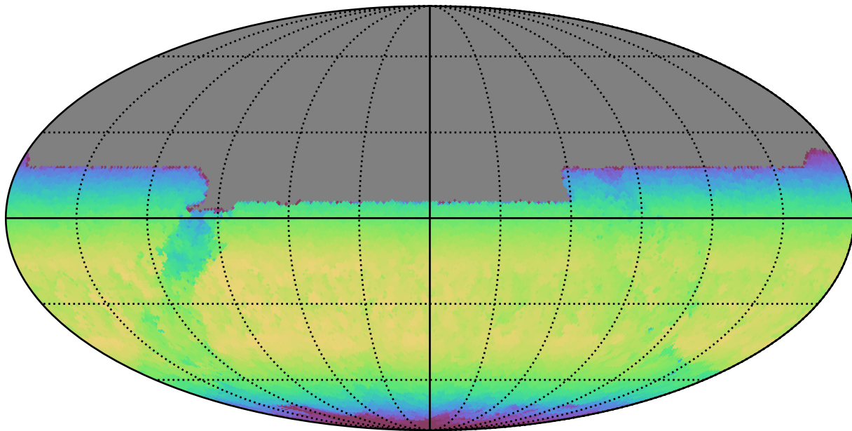
weather_cloudso12v3.4_10yrs All sky y band: Max skyBrightness
