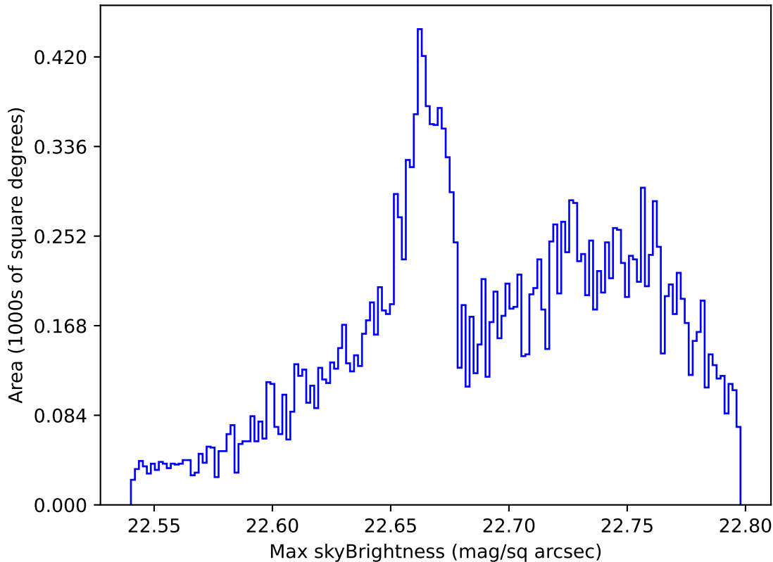
weather_cloudso12v3.4_10yrs All sky u band: Max skyBrightness
