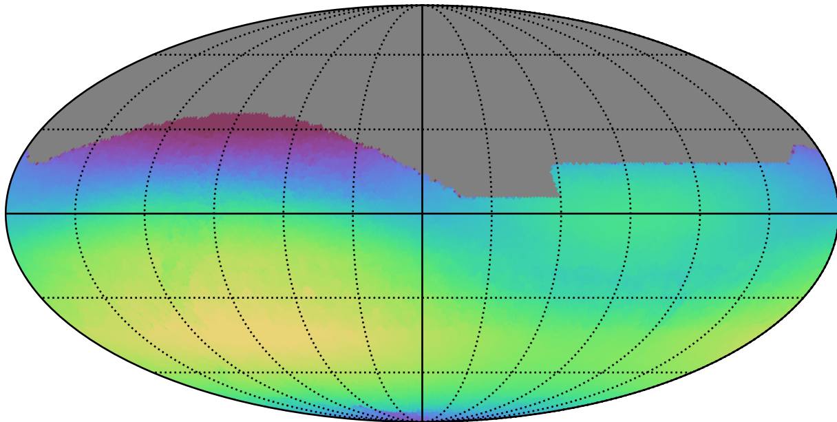
weather_cloudso12v3.4_10yrs All sky r band: Max skyBrightness
