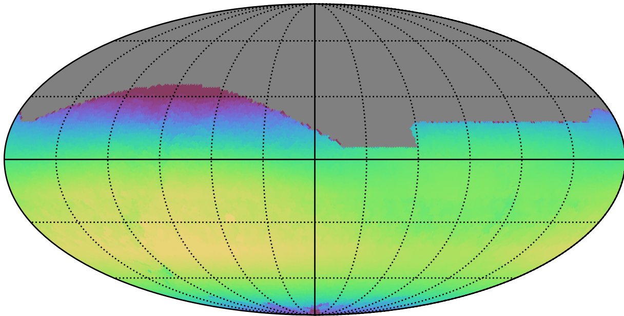
weather_cloudso12v3.4_10yrs All sky i band: Max skyBrightness
