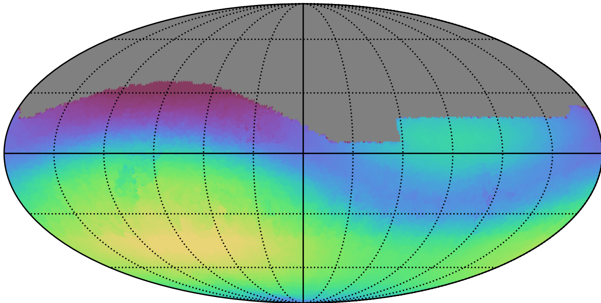
weather_cloudso12v3.4_10yrs All sky g band: Max skyBrightness
