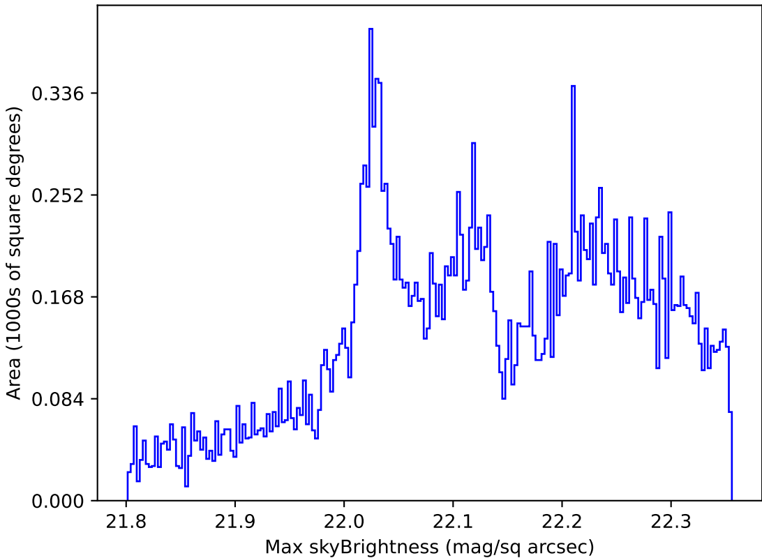
weather_cloudso12v3.4_10yrs All sky g band: Max skyBrightness
