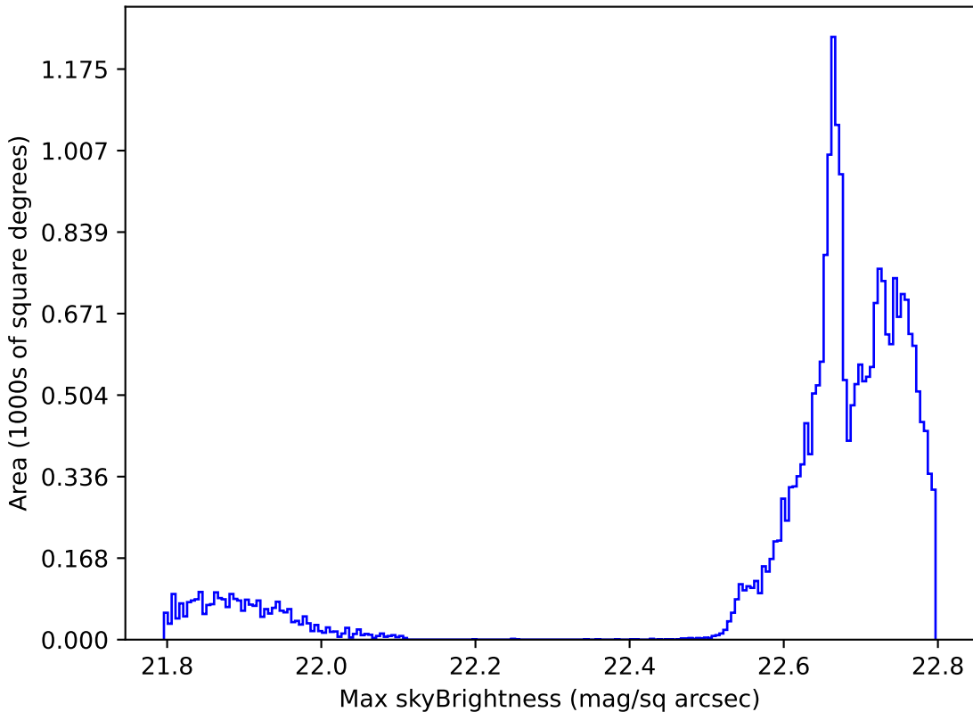
weather_cloudso12v3.4_10yrs All sky all bands: Max skyBrightness
