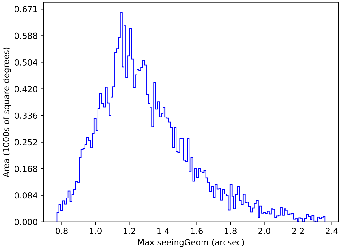
weather_cloudso12v3.4_10yrs Yr 1 z band: Max seeingGeom
