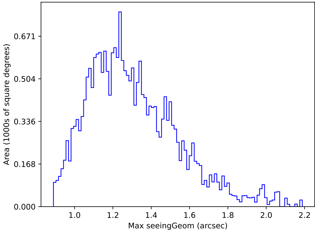
weather_cloudso12v3.4_10yrs Yr 1 y band: Max seeingGeom
