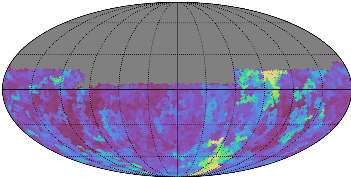
weather_cloudso12v3.4_10yrs Yr 1 u band: Max seeingGeom
