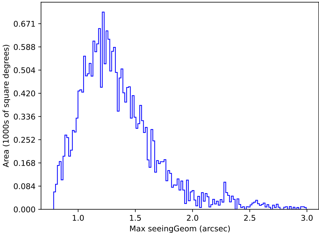
weather_cloudso12v3.4_10yrs Yr 1 u band: Max seeingGeom
