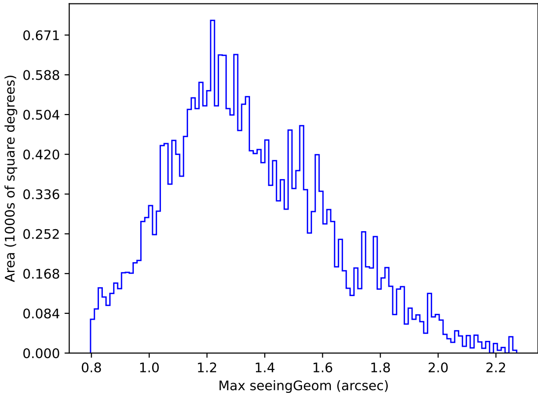
weather_cloudso12v3.4_10yrs Yr 1 r band: Max seeingGeom
