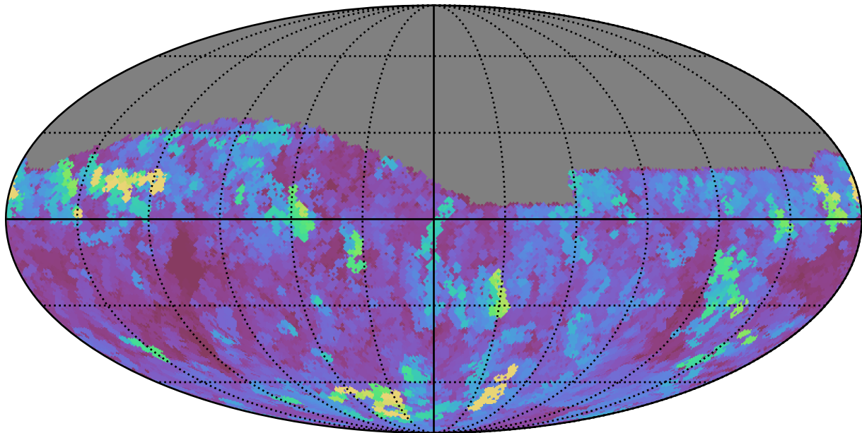
weather_cloudso12v3.4_10yrs Yr 1 i band: Max seeingGeom
