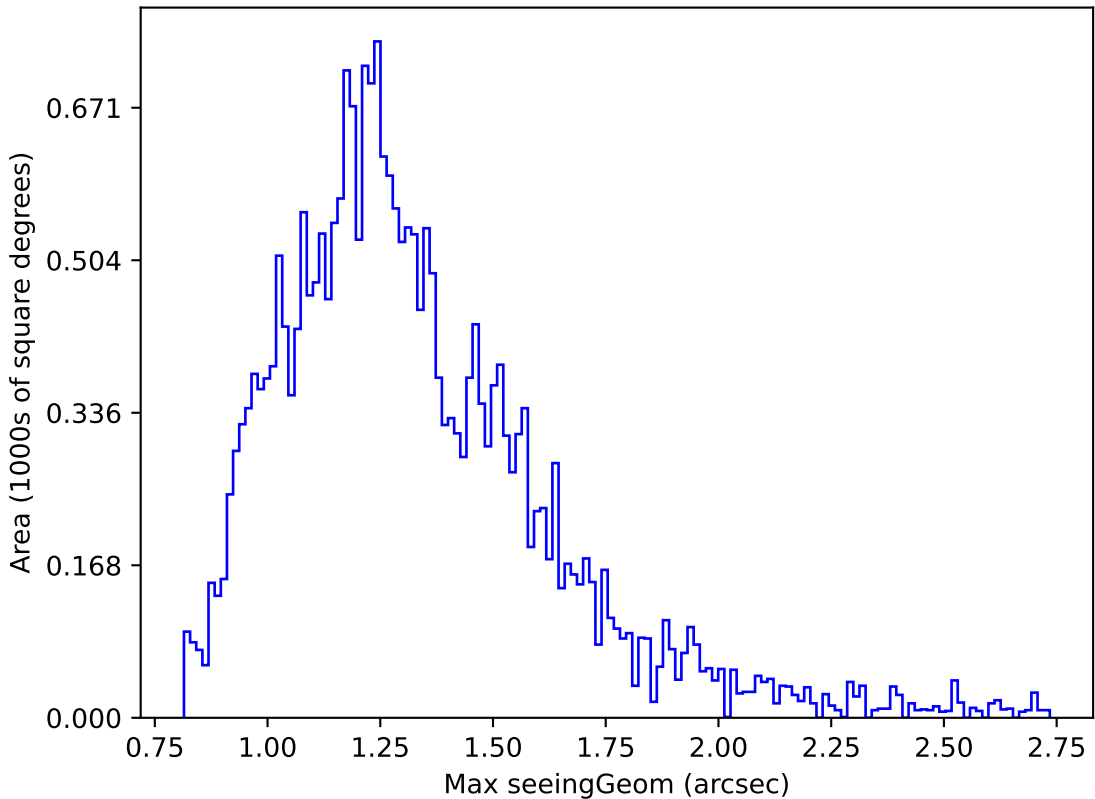
weather_cloudso12v3.4_10yrs Yr 1 i band: Max seeingGeom
