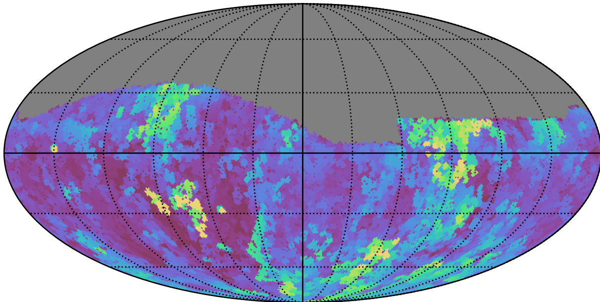
weather_cloudso12v3.4_10yrs Yr 1 g band: Max seeingGeom
