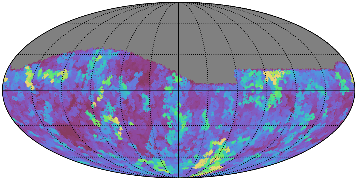
weather_cloudso12v3.4_10yrs Yr 1 all bands: Max seeingGeom
