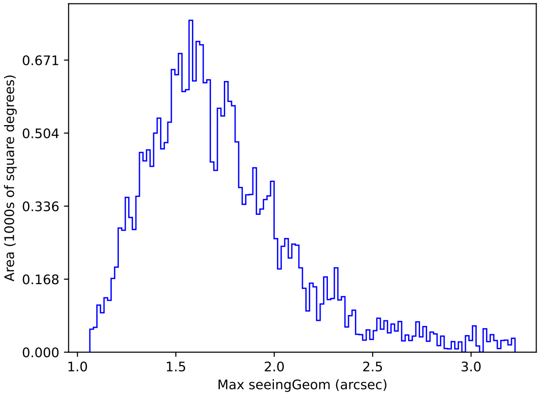
weather_cloudso12v3.4_10yrs Yr 1 all bands: Max seeingGeom
