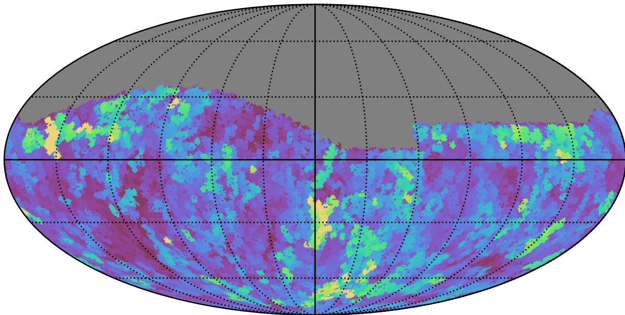
weather_cloudso12v3.4_10yrs Yr 1 z band: Max seeingEff
