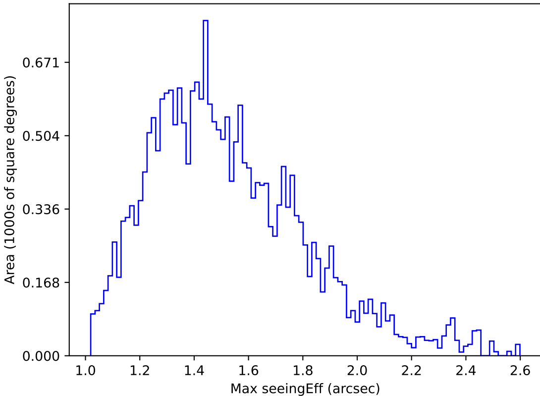
weather_cloudso12v3.4_10yrs Yr 1 y band: Max seeingEff
