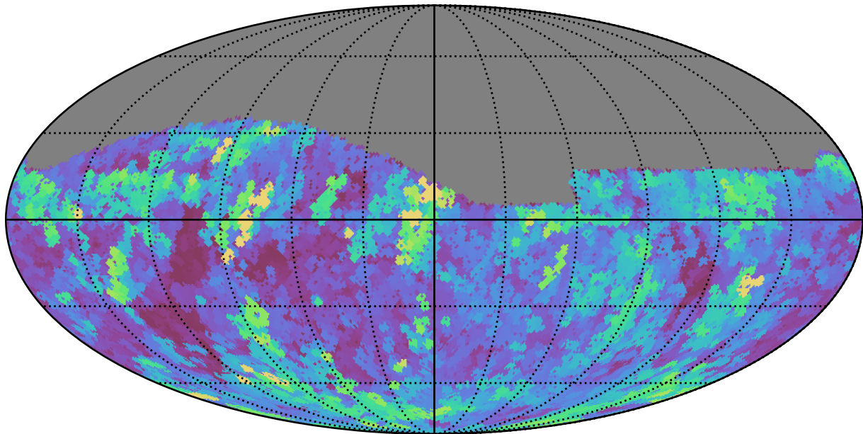
weather_cloudso12v3.4_10yrs Yr 1 r band: Max seeingEff
