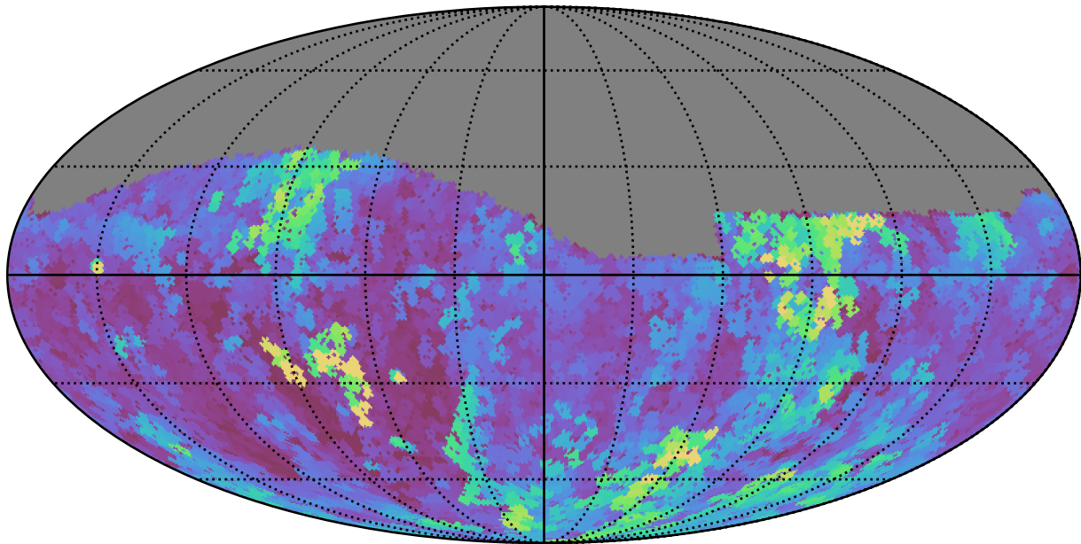
weather_cloudso12v3.4_10yrs Yr 1 g band: Max seeingEff
