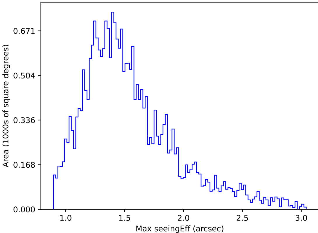
weather_cloudso12v3.4_10yrs Yr 1 g band: Max seeingEff
