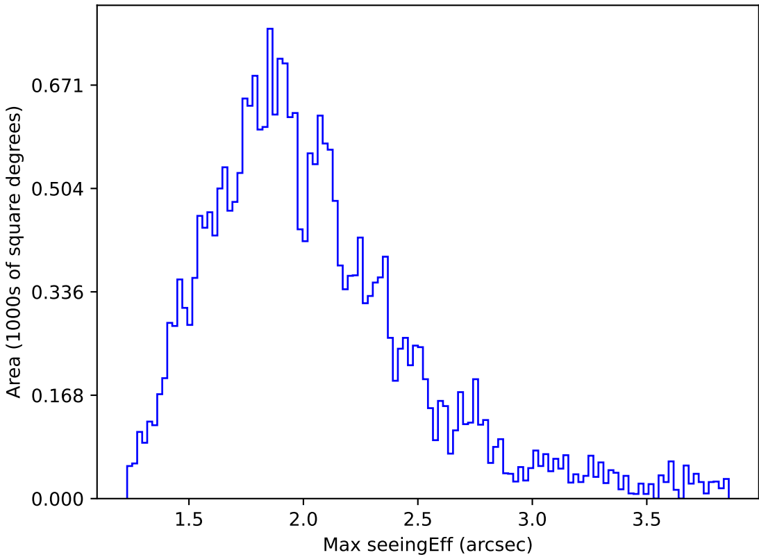
weather_cloudso12v3.4_10yrs Yr 1 all bands: Max seeingEff
