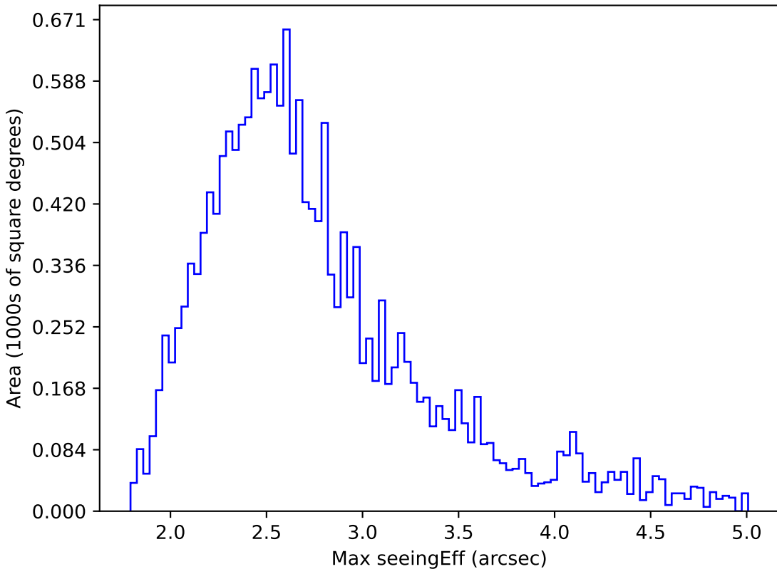
weather_cloudso12v3.4_10yrs WFD z band: Max seeingEff
