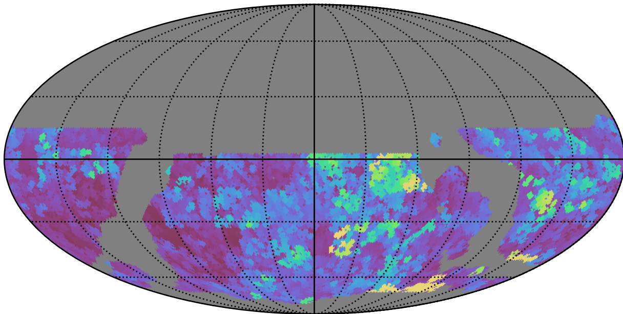
weather_cloudso12v3.4_10yrs WFD y band: Max seeingEff
