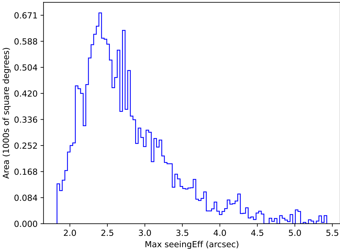
weather_cloudso12v3.4_10yrs WFD u band: Max seeingEff
