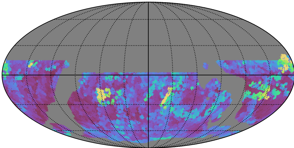
weather_cloudso12v3.4_10yrs WFD r band: Max seeingEff
