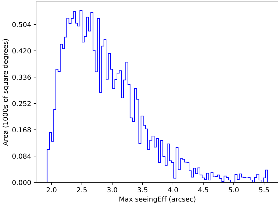
weather_cloudso12v3.4_10yrs WFD r band: Max seeingEff
