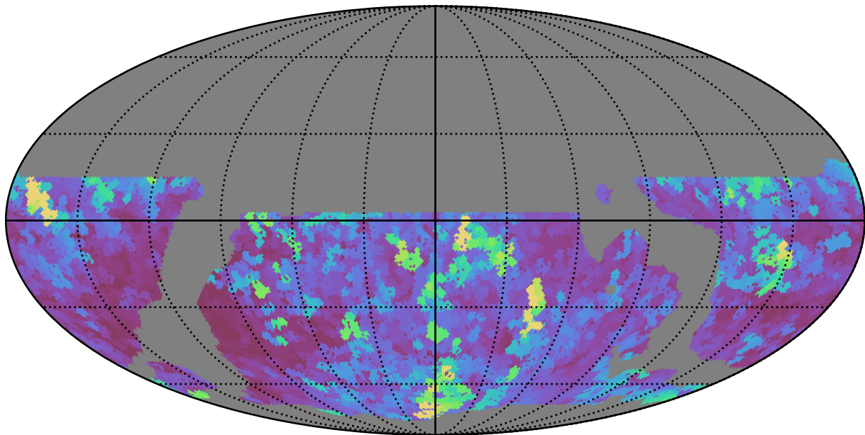
weather_cloudso12v3.4_10yrs WFD i band: Max seeingEff
