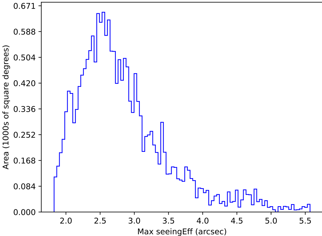
weather_cloudso12v3.4_10yrs WFD i band: Max seeingEff
