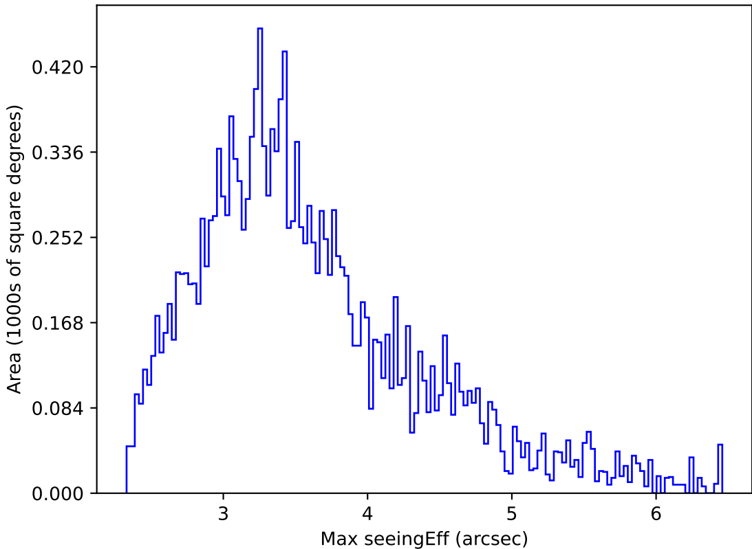
weather_cloudso12v3.4_10yrs WFD all bands: Max seeingEff
