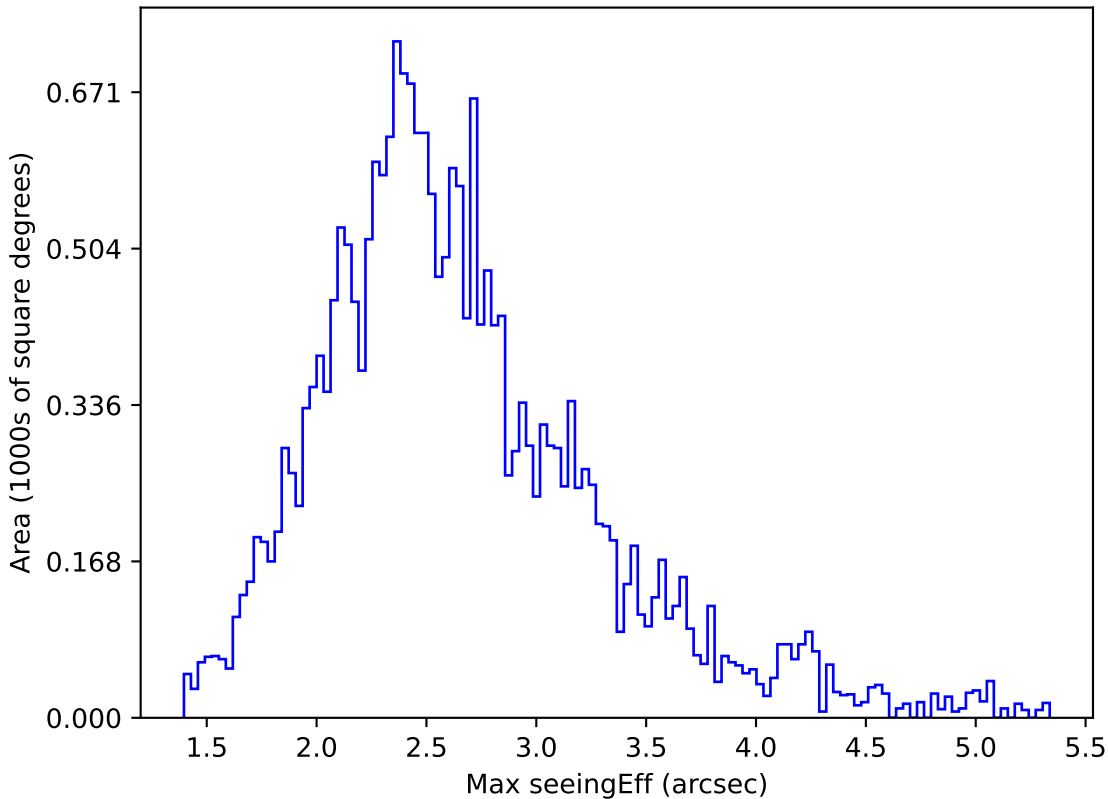
weather_cloudso12v3.4_10yrs All sky u band: Max seeingEff
