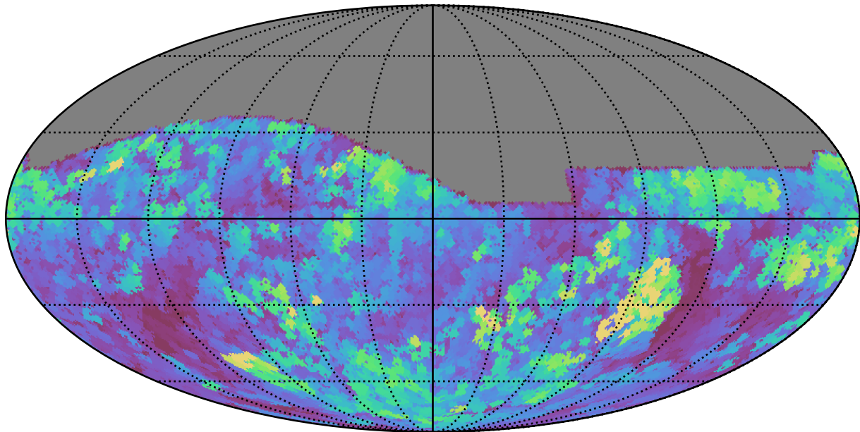
weather_cloudso12v3.4_10yrs All sky g band: Max seeingEff
