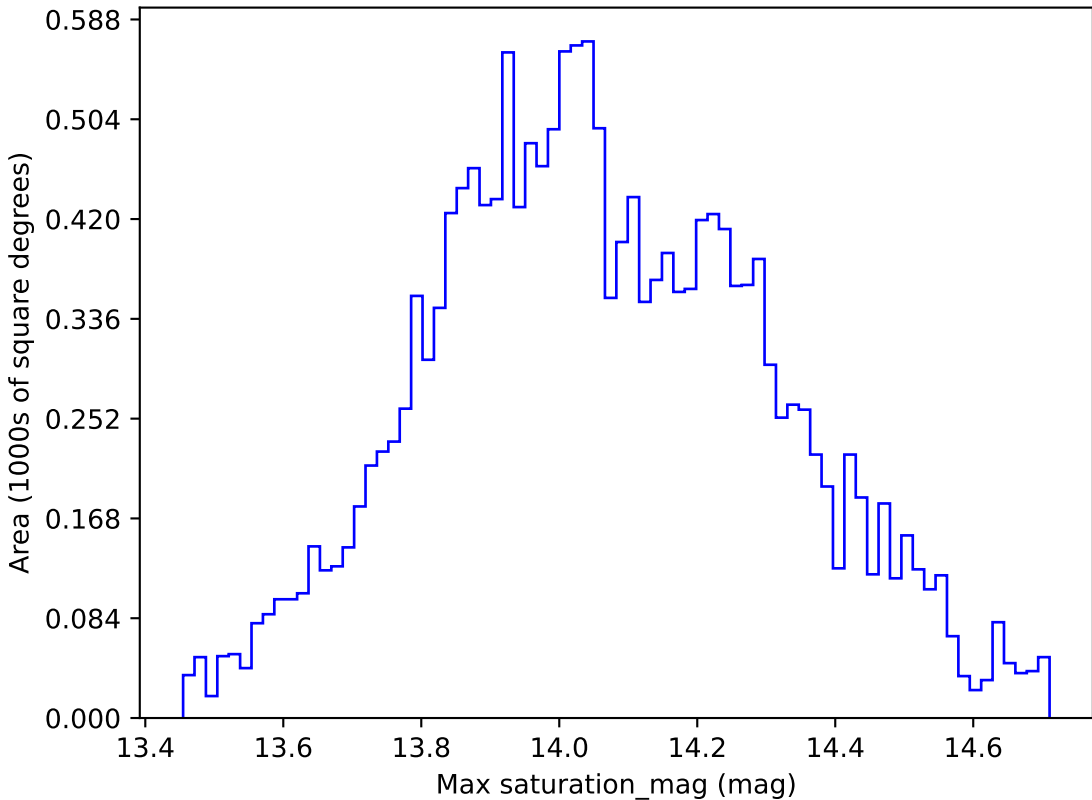
weather_cloudso12v3.4_10yrs WFD u band: Max saturation_mag
