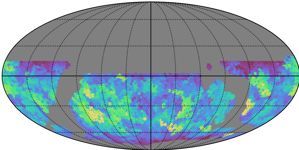
weather_cloudso12v3.4_10yrs WFD g band: Max saturation_mag
