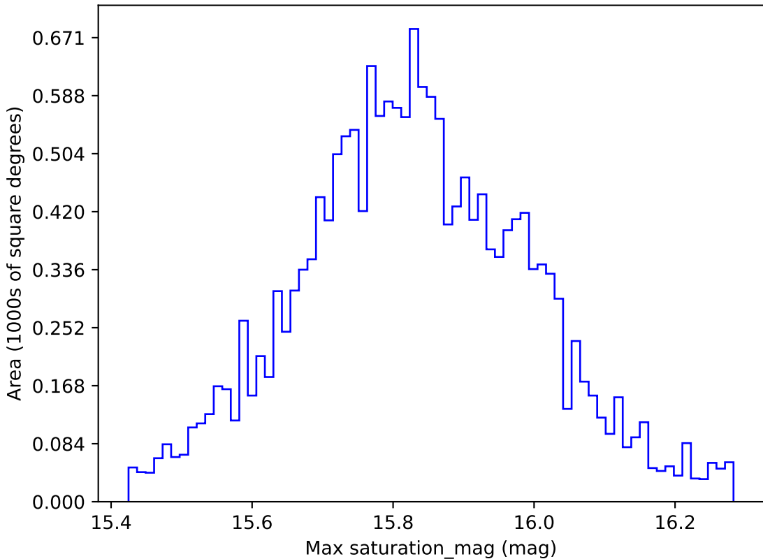
weather_cloudso12v3.4_10yrs WFD all bands: Max saturation_mag
