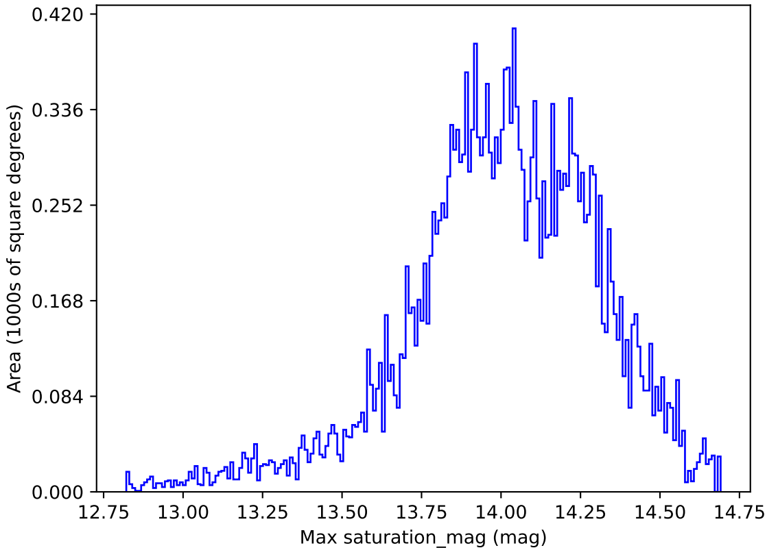
weather_cloudso12v3.4_10yrs All sky u band: Max saturation_mag
