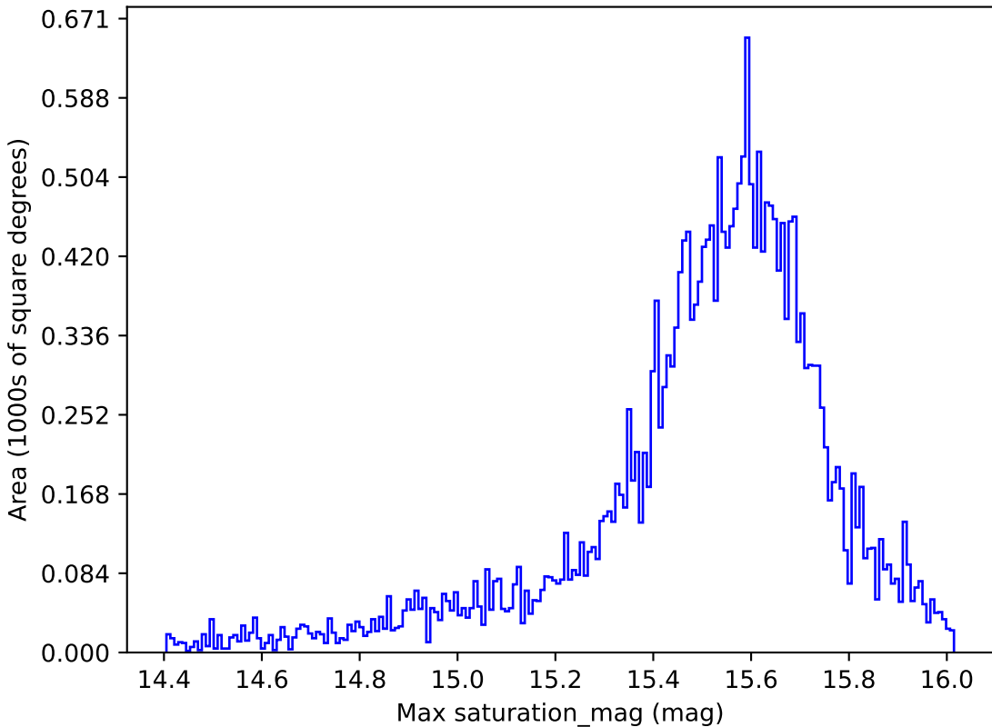
weather_cloudso12v3.4_10yrs All sky i band: Max saturation_mag
