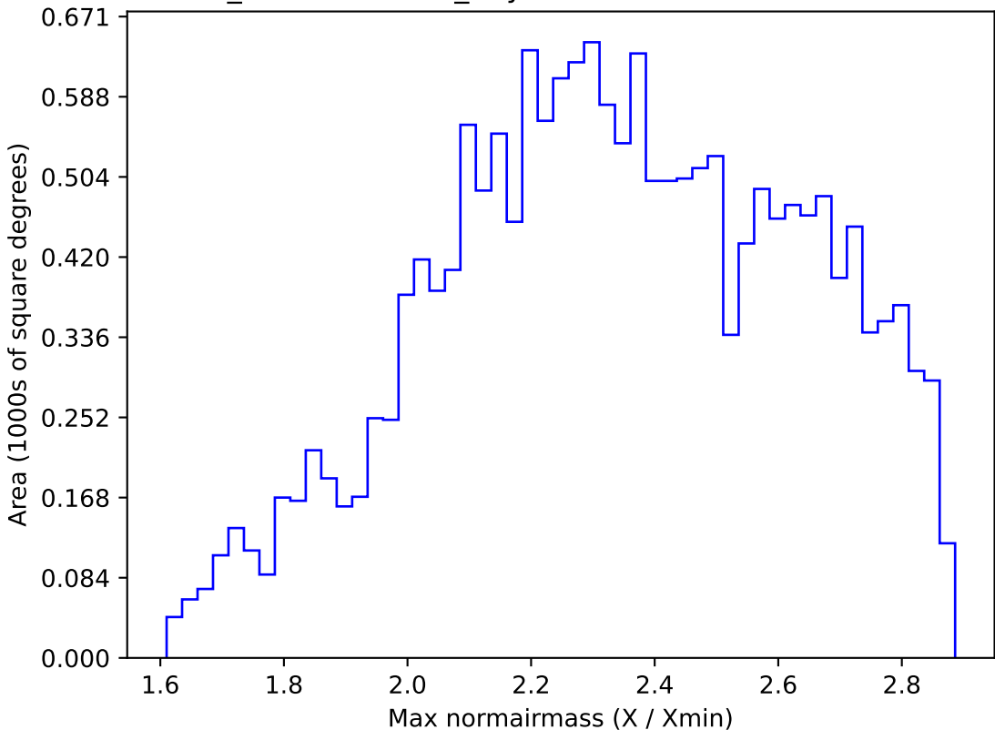
weather_cloudso12v3.4_10yrs WFD z band: Max normairmass
