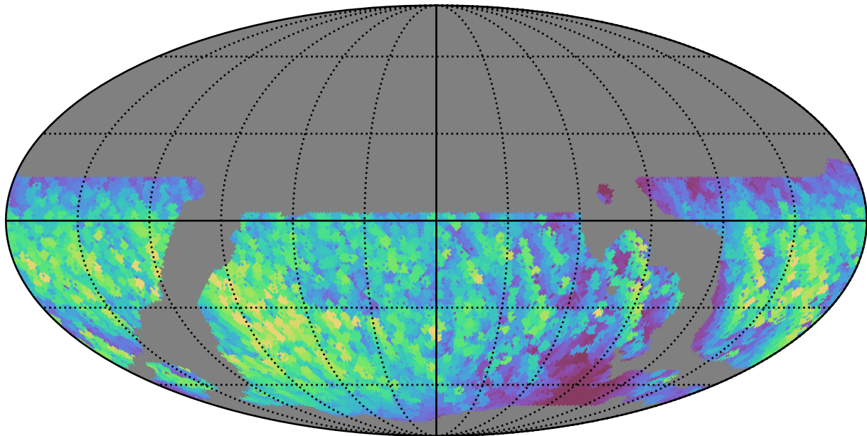
weather_cloudso12v3.4_10yrs WFD y band: Max normairmass
