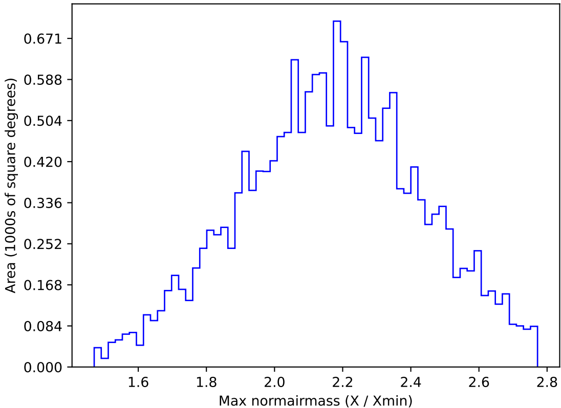
weather_cloudso12v3.4_10yrs WFD y band: Max normairmass
