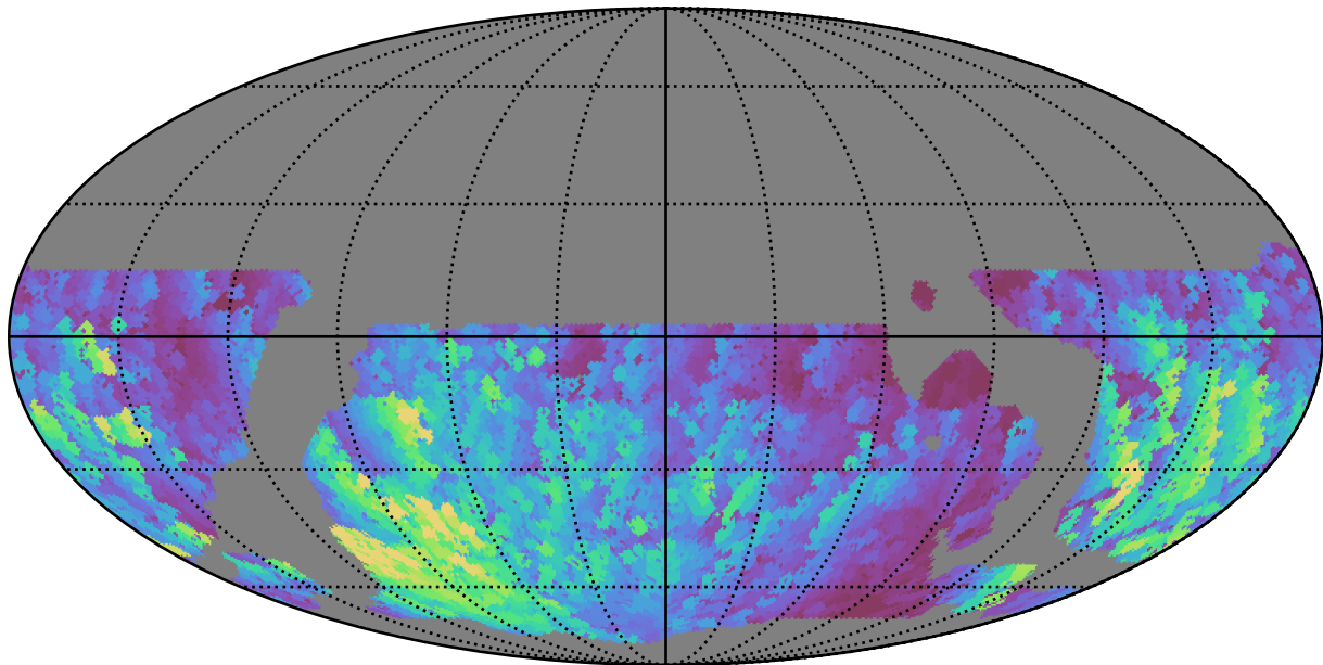
weather_cloudso12v3.4_10yrs WFD u band: Max normairmass
