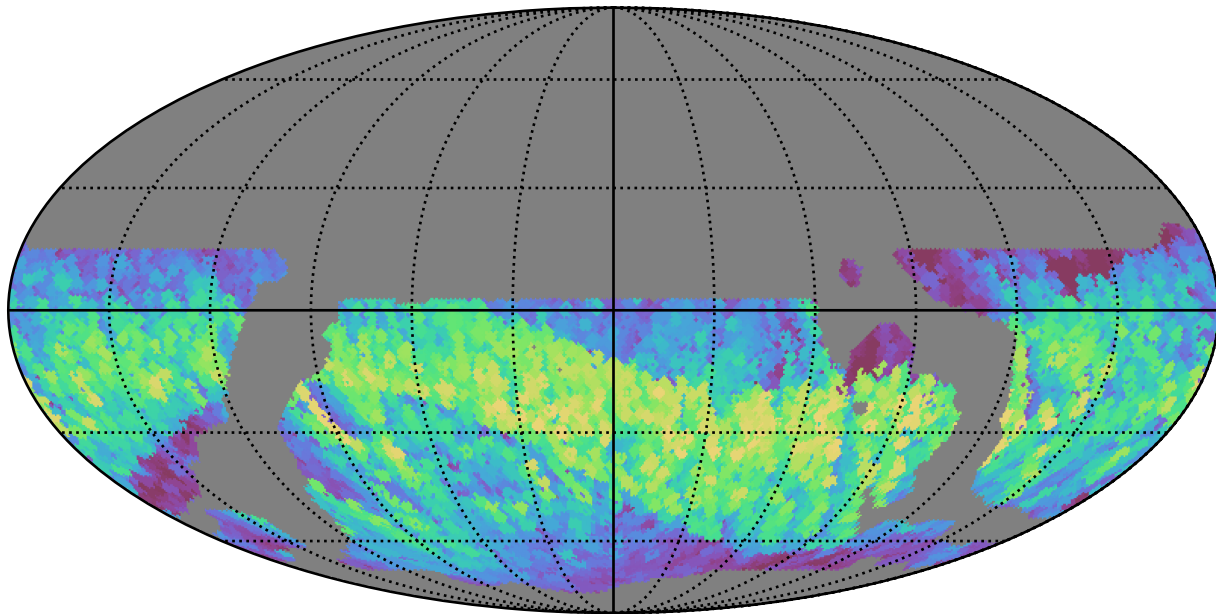
weather_cloudso12v3.4_10yrs WFD i band: Max normairmass
