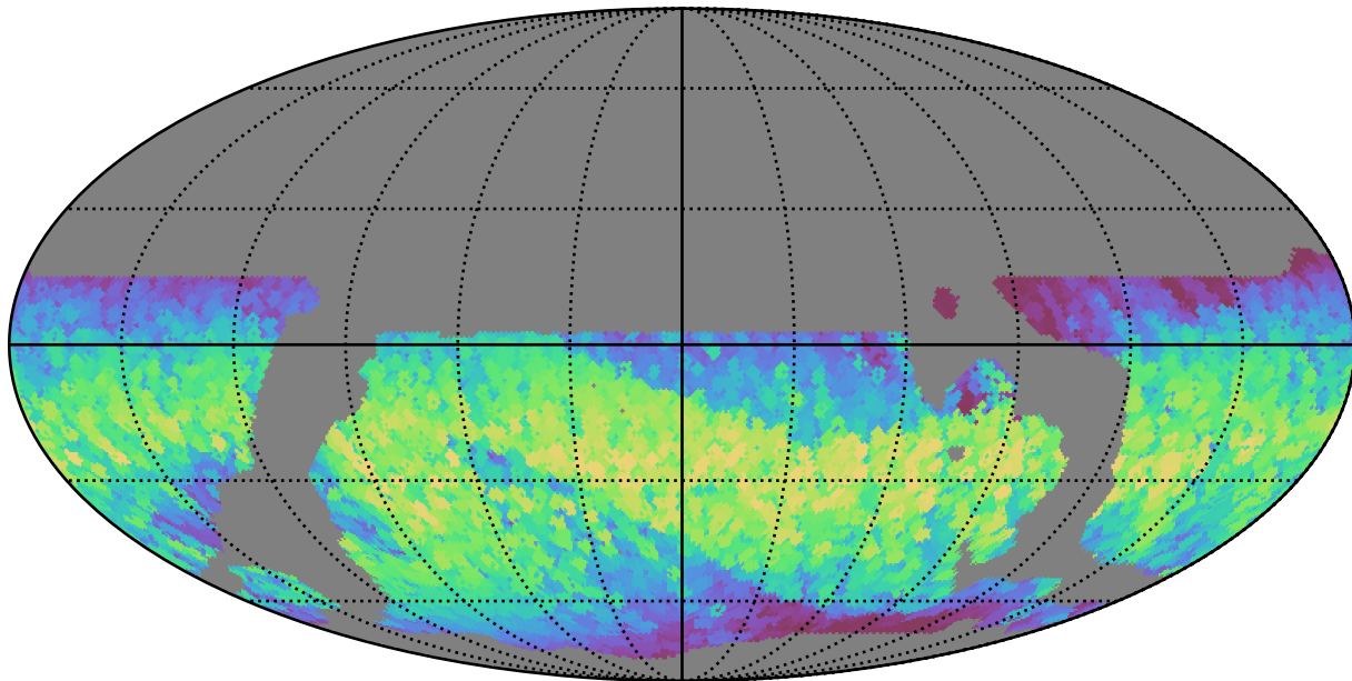
weather_cloudso12v3.4_10yrs WFD all bands: Max normairmass
