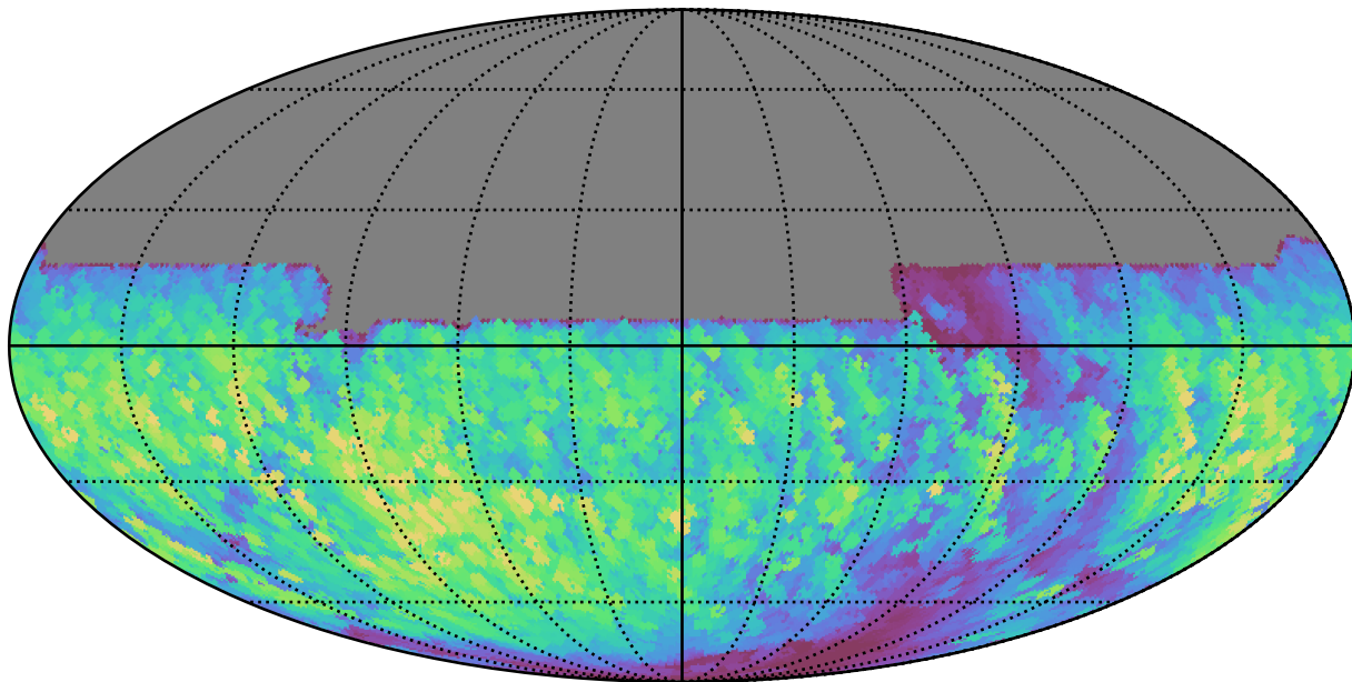
weather_cloudso12v3.4_10yrs All sky y band: Max normairmass
